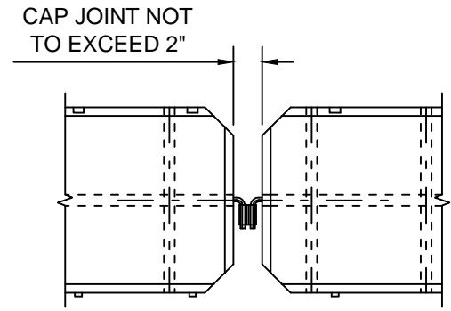
TYPICAL MAT CONNECTION ENLARGED PLAN VIEW
