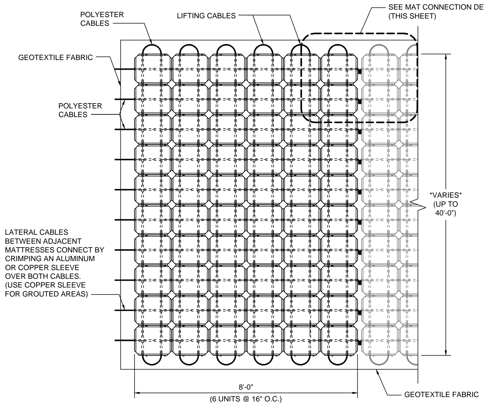
PARALLEL ACBM PLAN VIEW
