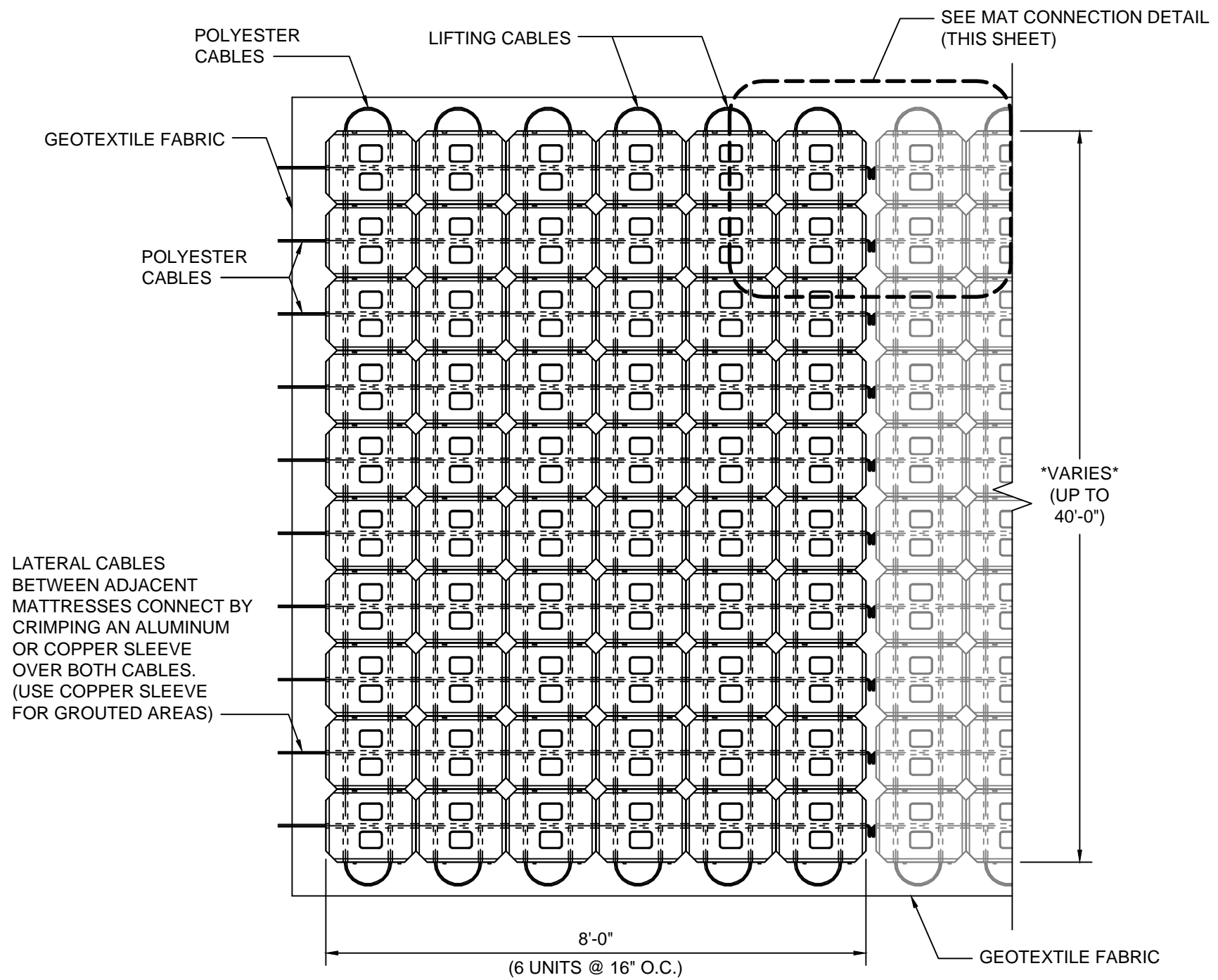
PARALLEL ACBM PLAN VIEW
