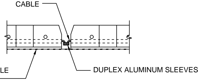
TYPICAL MAT CONNECTION ENLARGED SECTION VIEW
