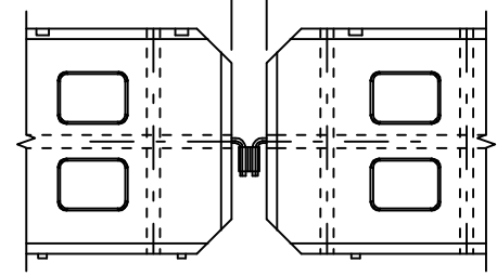
TYPICAL MAT CONNECTION ENLARGED PLAN VIEW
