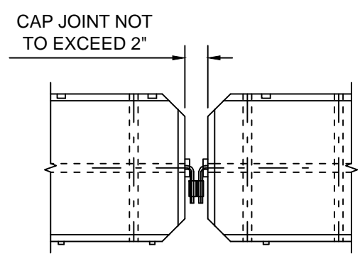
TYPICAL MAT CONNECTION ENLARGED PLAN VIEW
