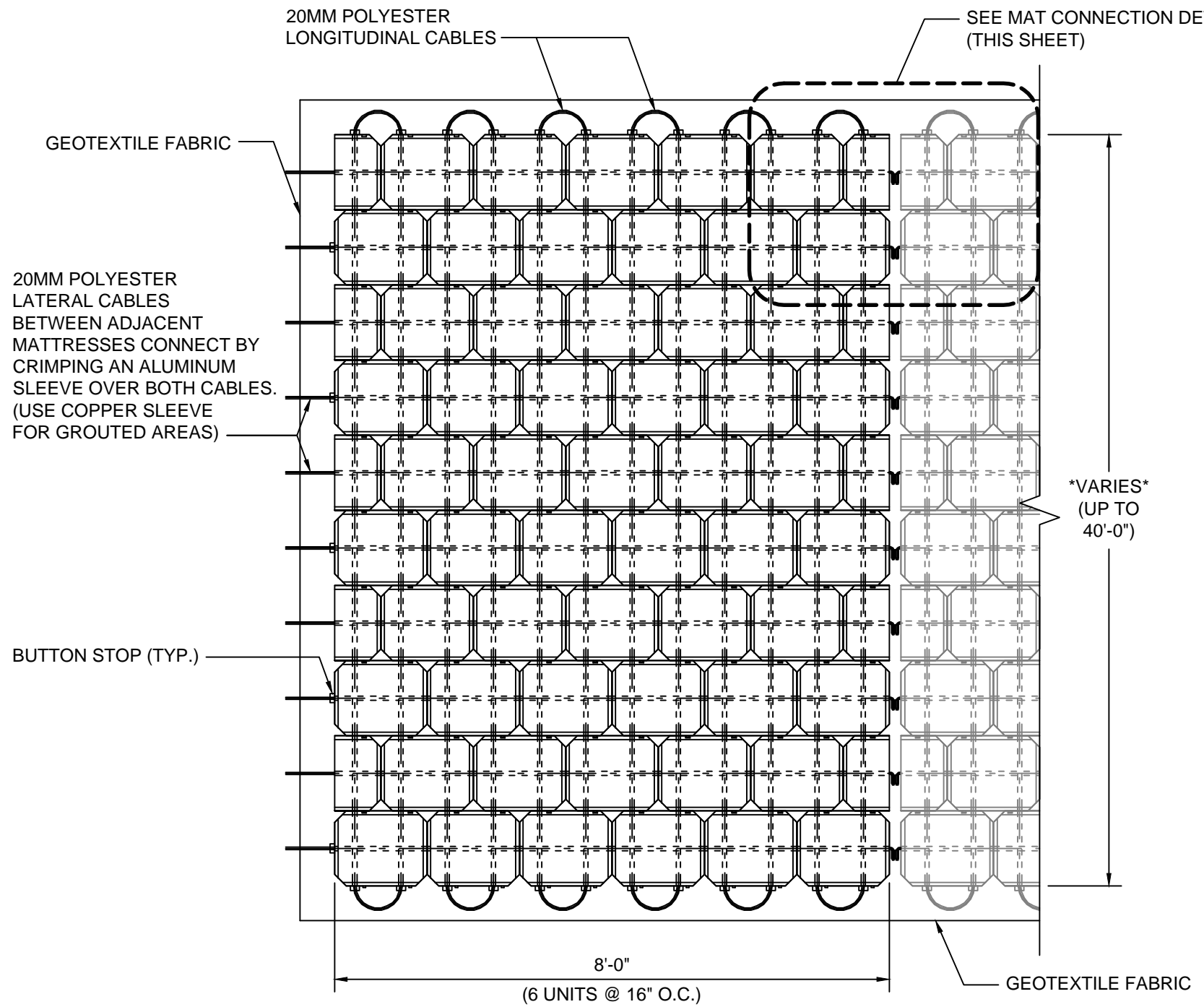
STAGGERED ACBM PLAN VIEW
