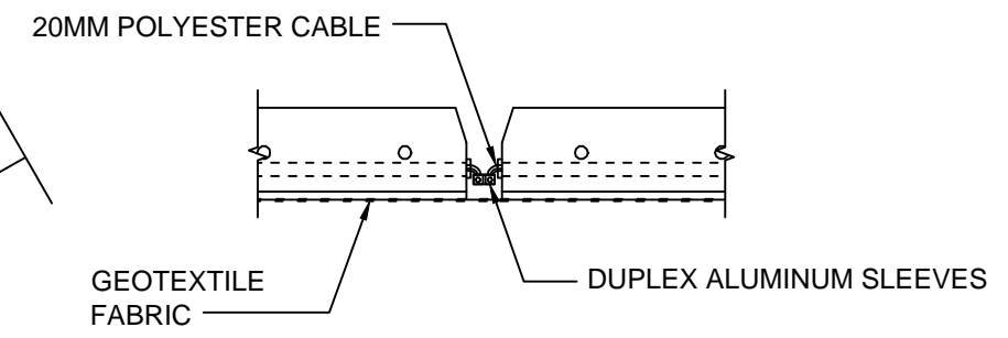
TYPICAL MAT CONNECTION ENLARGED SECTION VIEW
