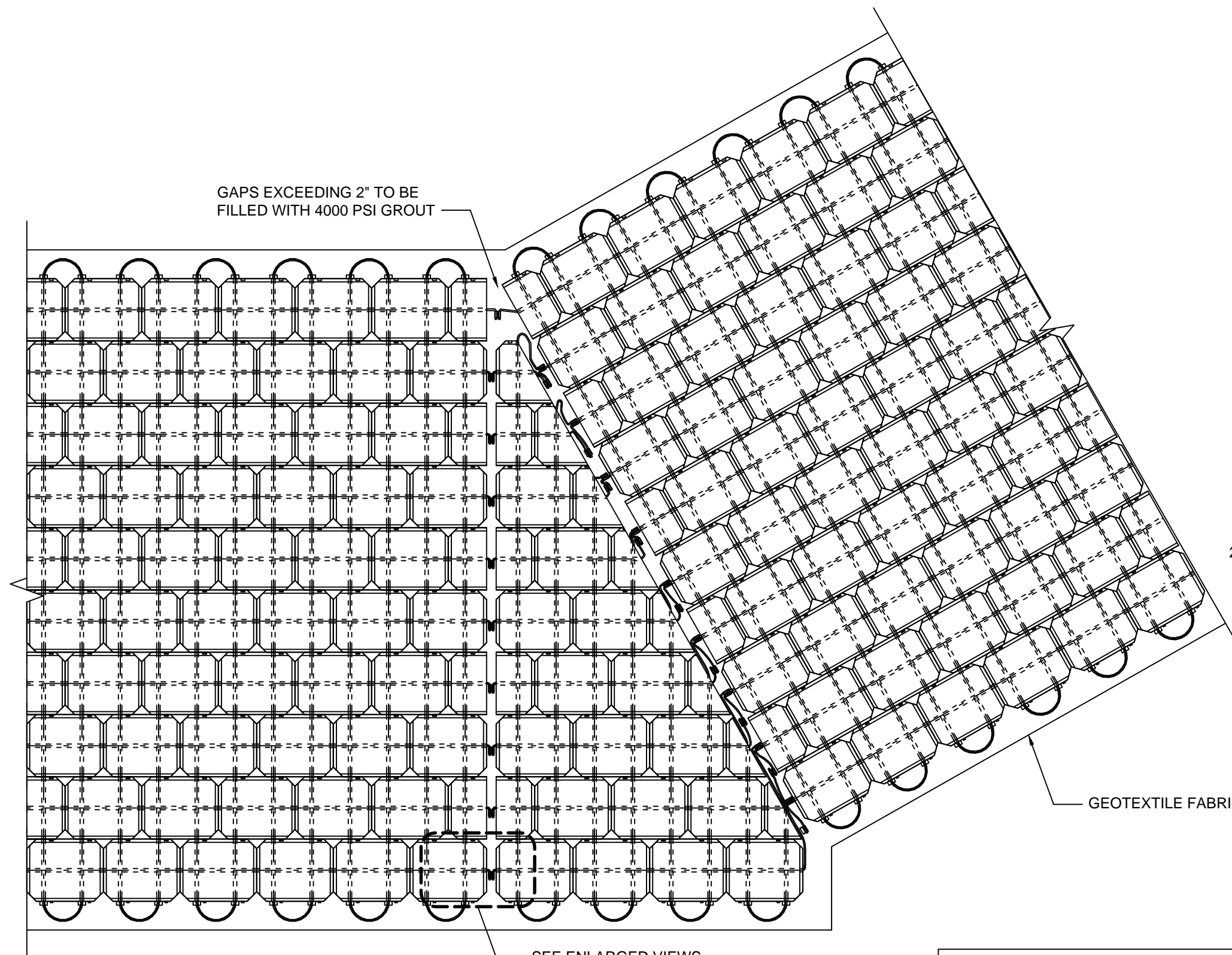
ANGLED ACBM CONNECTION PLAN VIEW
