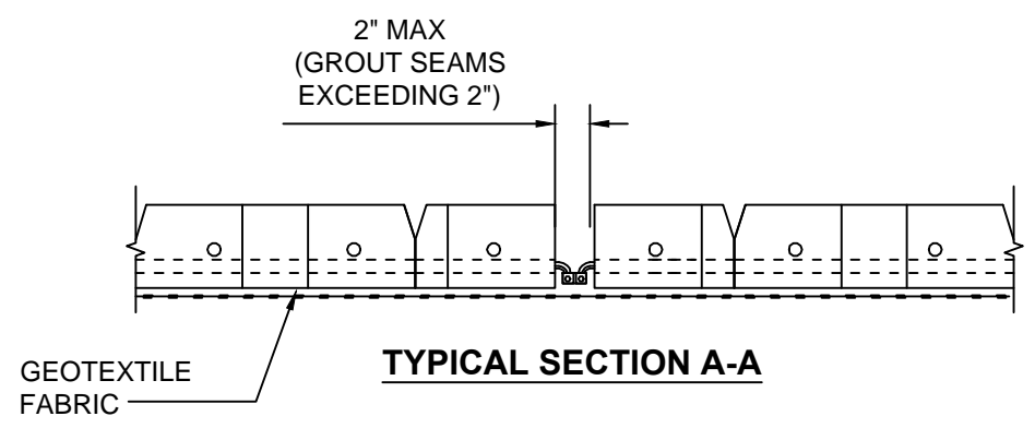
TYPICAL CONNECTION OF TWO MATS
