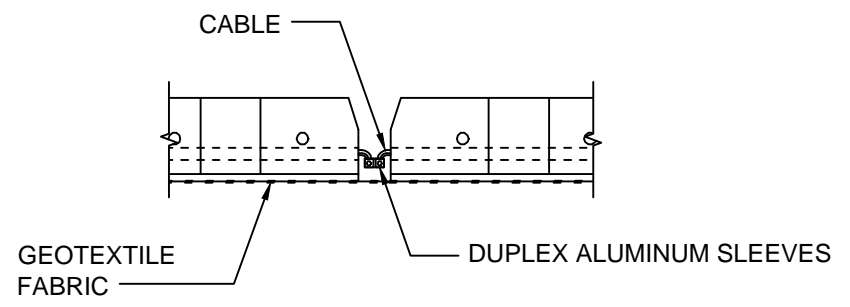
TYPICAL MAT CONNECTION ENLARGED SECTION VIEW
