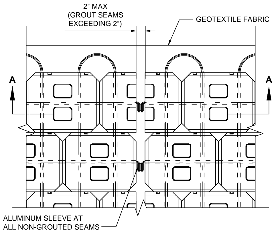
TYPICAL CONNECTION OF TWO MATS
