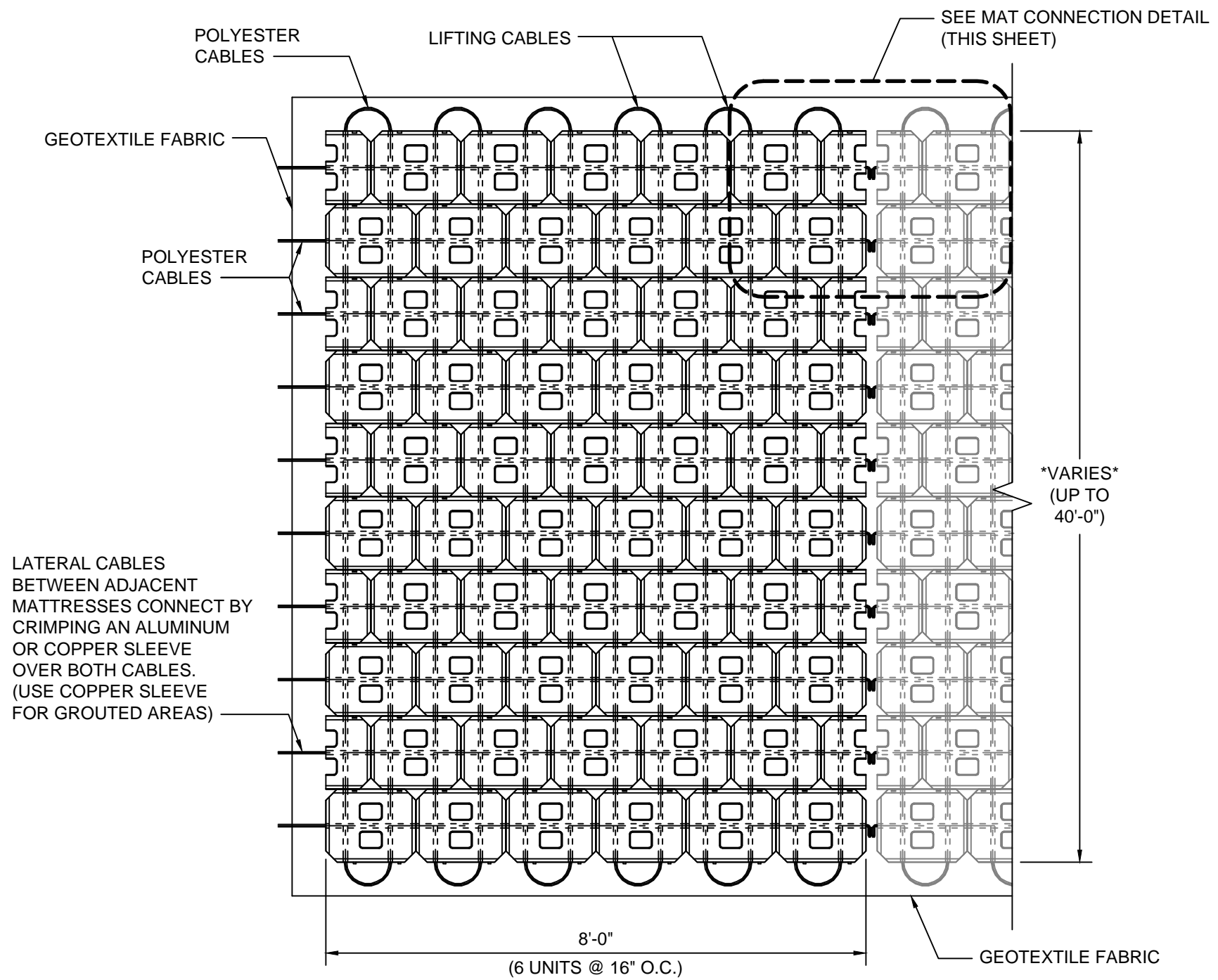
STAGGERED ACBM PLAN VIEW
