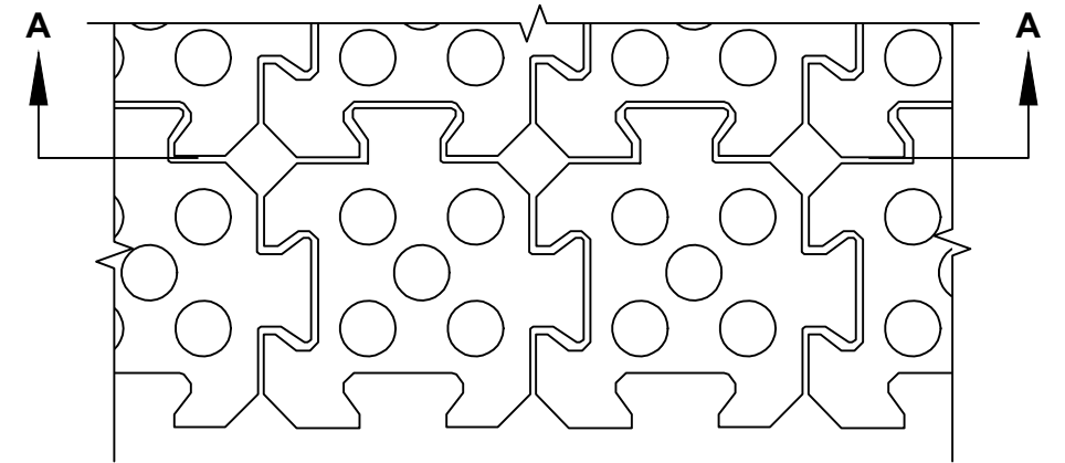
TYPICAL MAT CONNECTION ENLARGED PLAN VIEW
