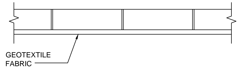
TYPICAL MAT CONNECTION ENLARGED SECTION VIEW
